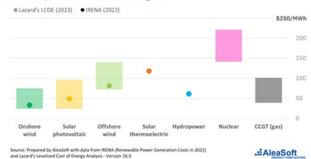
Levelized Cost of Electricity (LCOE) LCOE comparison of different technologies
